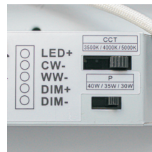
Tuning Switches Inside Housing
